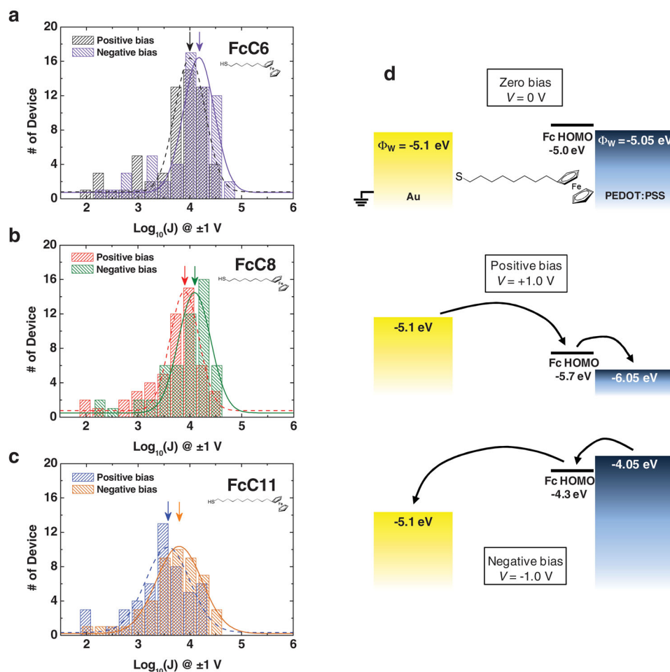
Figure 3. a,b,c) Histograms of the logarithmic current densities measured at \pm 1 \text{ V} for FcC6, FcC8, and FcC11 molecular devices. The arrows indicate the mean value of the logarithmic current density of each molecular device at both bias polarities. d) The proposed energy band diagram for the molecular junctions at three bias conditions (0, 1, and -1 \text{ V} ). Arrows depict the charge conduction through the molecular junction. The HOMO of ferrocene and the Fermi level of Au were adopted from the literature, while the Fermi level of PEDOT:PSS was measured by Kelvin Probe measurements.
