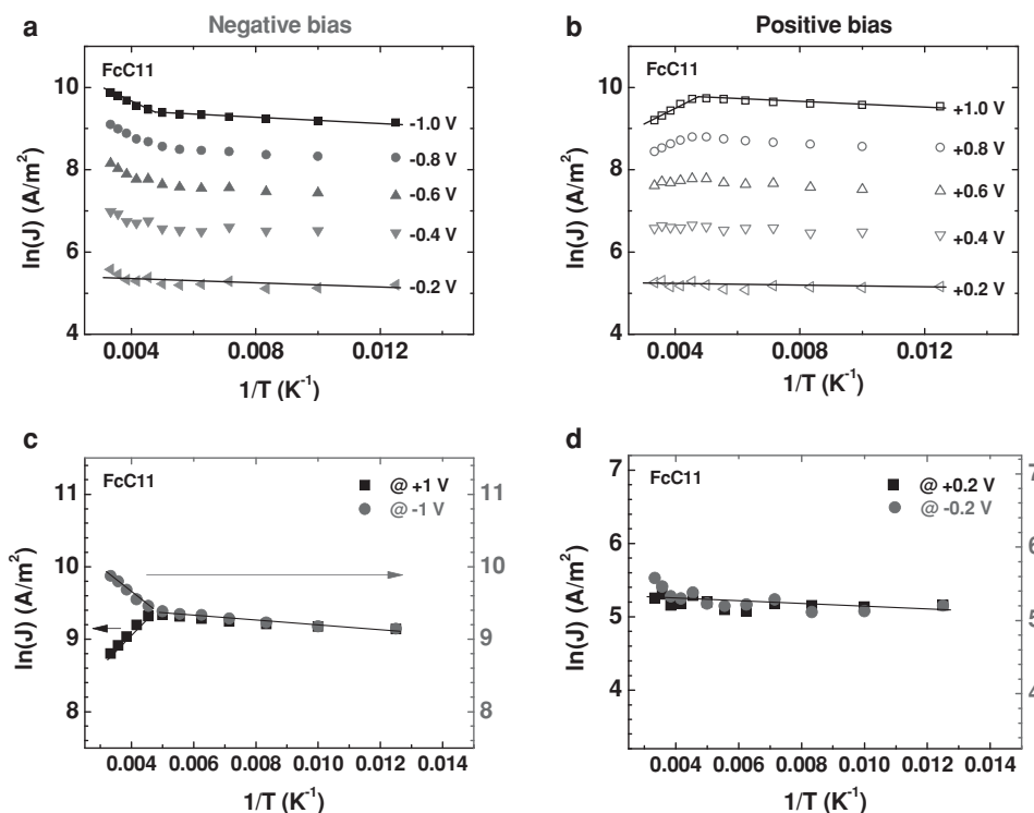
Figure 5. a,b) Arrhenius plots of \ln(J) versus 1/T for an FcC11 molecular device at different a) negative and b) positive biases. c,d) Arrhenius plot of the data measured at c) \pm 1 \text{ V} and d) \pm 0.2 \text{ V} from plot (a) and (b), respectively.
